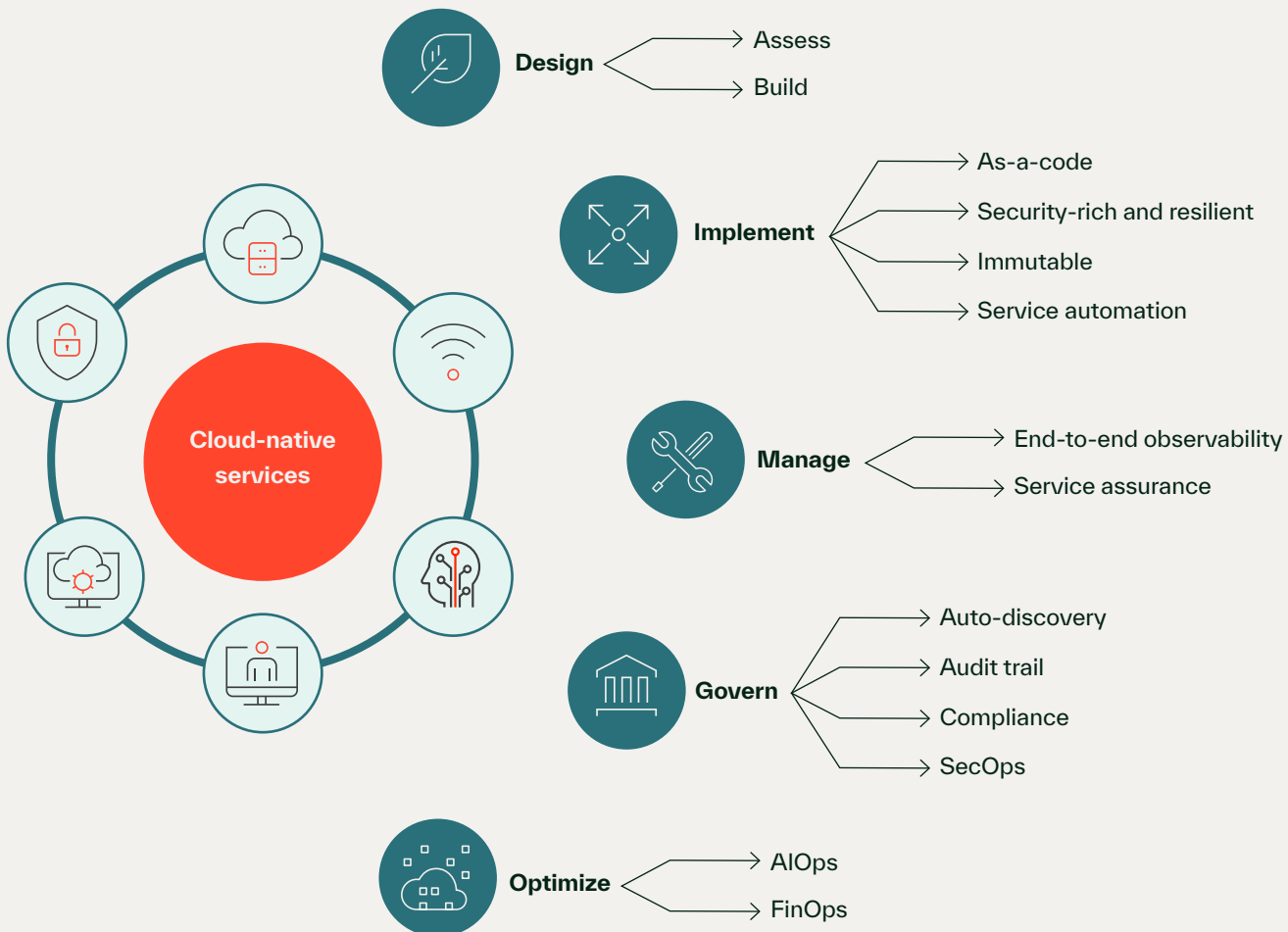
Figure 1. Enabling cloud-native operational framework
